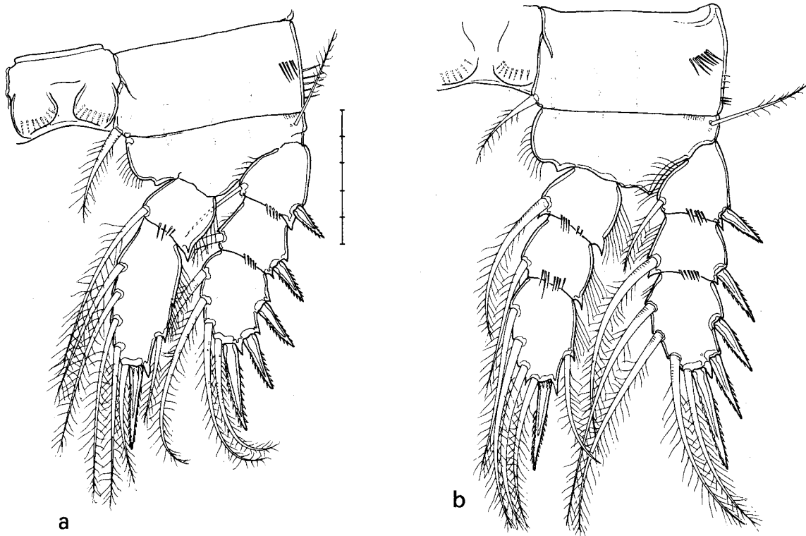
Fig. 3. Diacyclops cohabitatus female: a) P2 ; b) P3. Scale bars : 50 \mu m.
