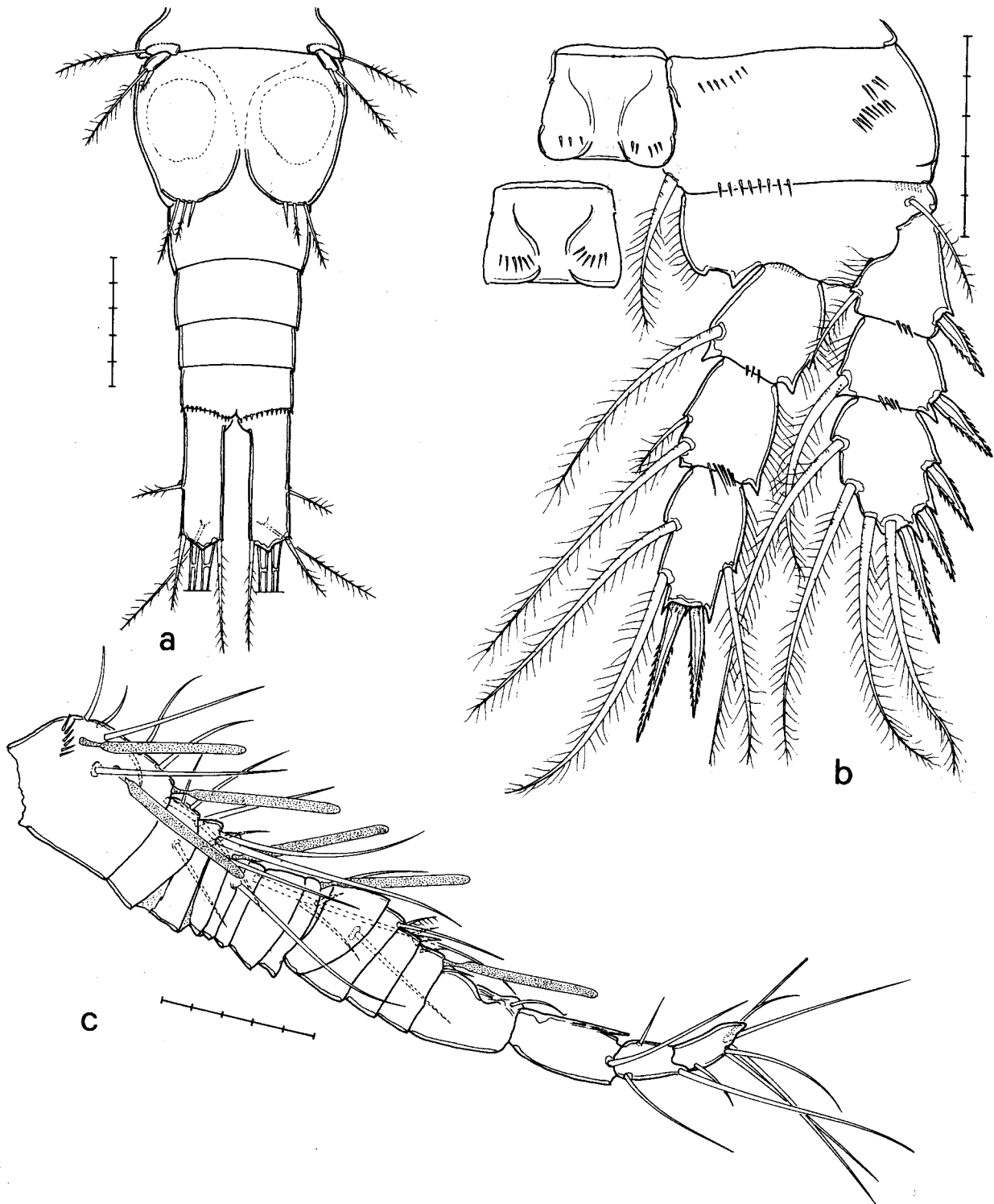
Fig. 4. Diacyclops cohabitatus male (a,c) and female (b) : a) abdomen and caudal rami, ventral view ; b) P4 ; c) antennule. Scale bars : 50 \mu m.
