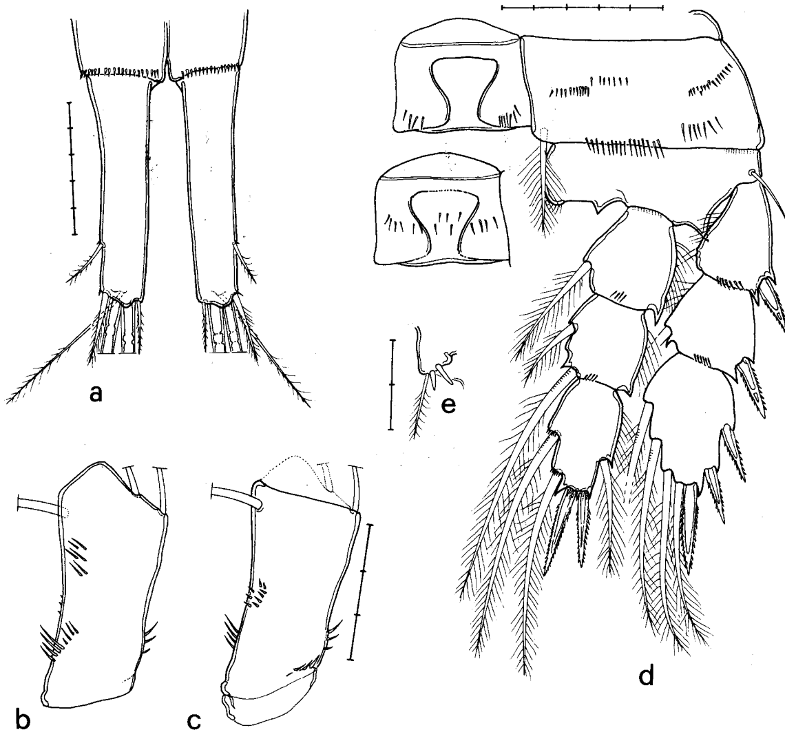
Fig. 5. Diacyclops languidoides goticus female : a) caudal rami, ventral view; b) antennary basis with spinule pattern, caudal side ; c) ibidem, frontal side ; d) P4 ; e) P6. Scale bars : 50 \mu m (a, d), 30 \mu m (b,c), 20 \mu m (e).
