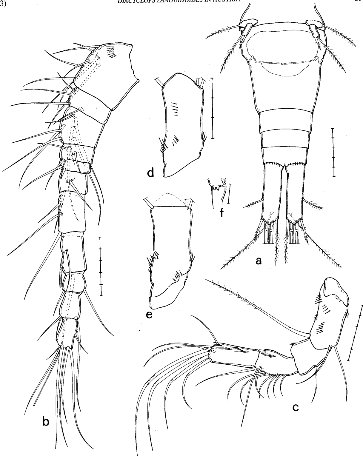
Fig. 1. Diacyclops cohabitatus female : a) abdomen and caudal rami, ventral view ; b) antennule ; c) antenna ; d) antennary basis with spinule pattern, caudal side ; e) ibidem, frontal side ; f) P6. Scale bars : 50 \mu m (a,b,c), 30 \mu m (d,e), 10 \mu m (f).
